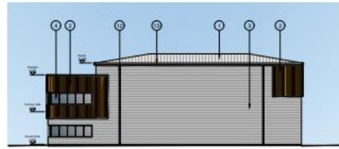
WESTERN ELEVATION
